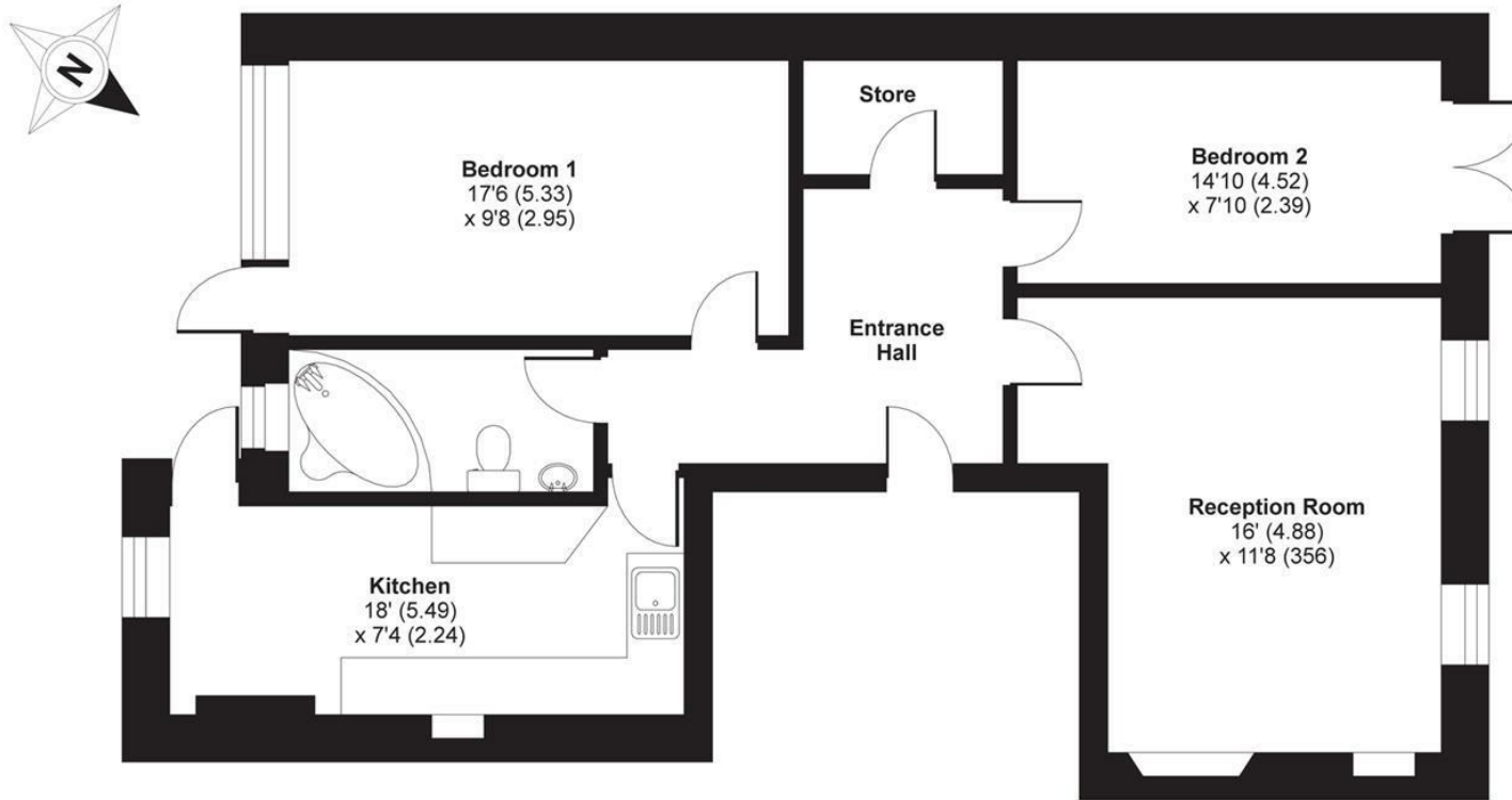
GROUND FLOOR
